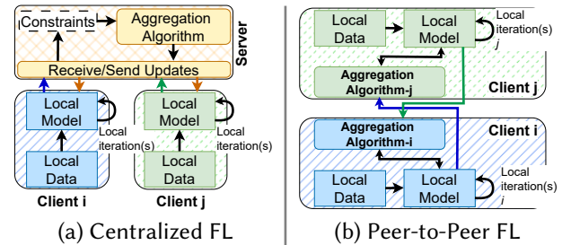
Figure 1. Overview of (a) Centralized and (b) Peer-to-Peer Federated Learning schemes.
