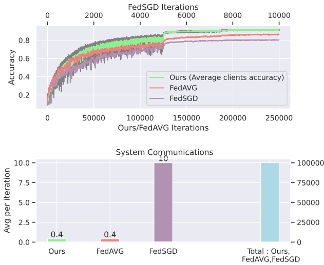
Figure 5. Accuracy and Communication cost : 5 clients - Cifar10.
